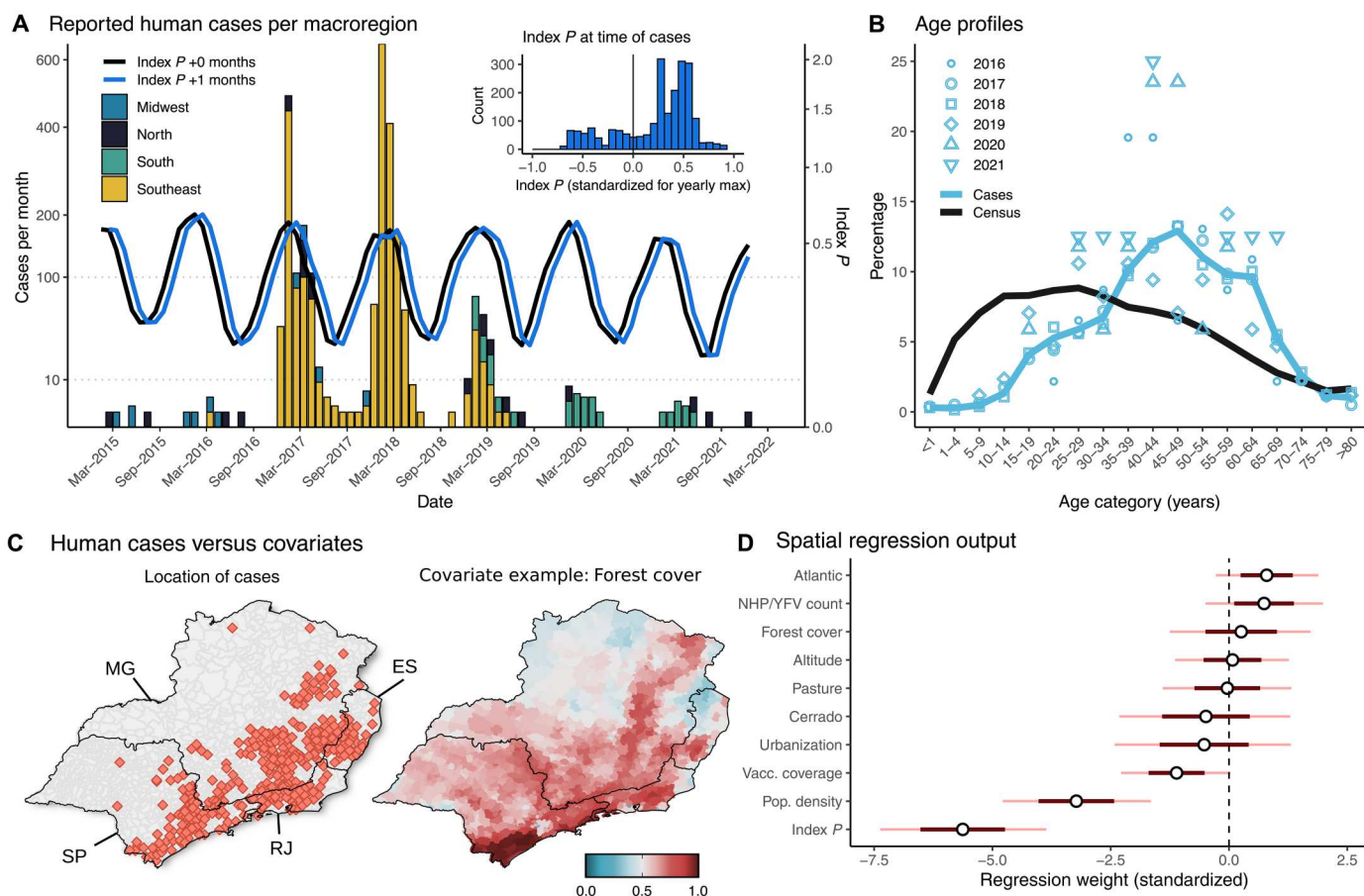
Fig. 1. Human incidence of YFV in Brazilian macroregions, 2015–2022. (A) Time series of monthly reported human cases in four Brazilian macroregions (those reporting the majority of cases) and monthly mosquito-viral suitability measure (index P ) aggregated (mean) across the macroregions. Index P is calibrated to YFV and Aedes aegypti , interpreted as spillover risk, and presented here index P is presented by the lines as baseline (black) and shifted by +1 month (blue). The inset plot shows the distribution (y axis) of human cases according to the value of index P (x axis) extracted at each time point of reported human YFV cases (shifted +1 month, standardized by yearly maximum). (B) Age distribution of human cases across the years (light blue) versus Census 2010 data (black), both aggregated across the Southeast and South macroregions. (C) Spatial distribution of human cases (red filled points) and one example of a spatial covariate (forest cover) used for modeling the Southeast macroregion. For all covariates, see fig. S1. Covariates were normalized by their maximum for visualization, with covariates population density, Atlantic and NHP cases first transformed with \log_{10} (color scale in the bottom right). Spatial boundaries (black) are states: São Paulo (SP), Espírito Santo (ES), Minas Gerais (MG), Rio de Janeiro (RJ). (D) Marginal posterior distributions (standardized to appear on the same scale) for individual regression weights for the 10 covariates explored.
