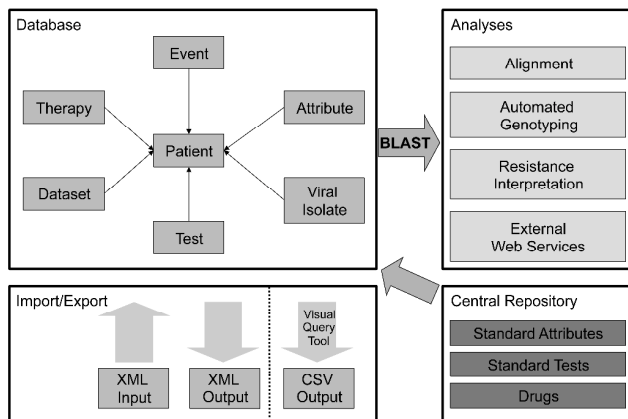
Figure 1: An overview of RegaDB's database entities and functionalities.
